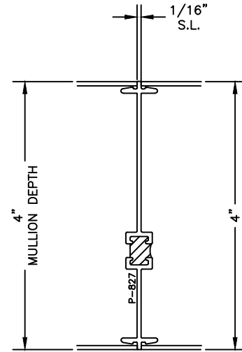
P-827 SNAP MULLION (1/16")
