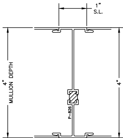
P-826 SNAP MULLION (1")
