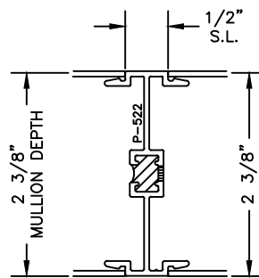
P-522 SNAP MULLION
