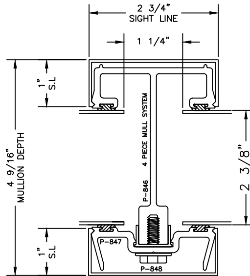
4 PC. MULLION
