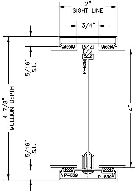
4 PC. MULLION
