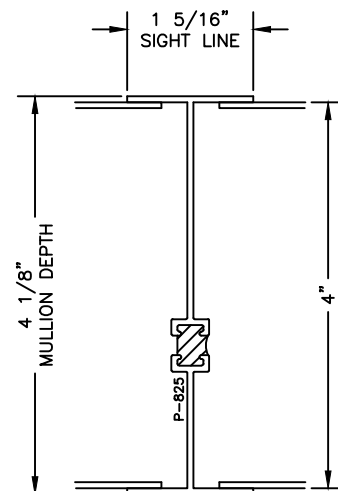
P-825 MULLION
