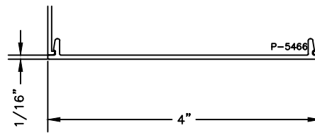
4" CAULKING BACKER
