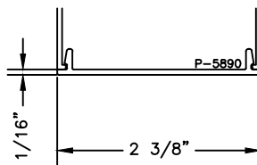
2 3/8" CAULKING BACKER
