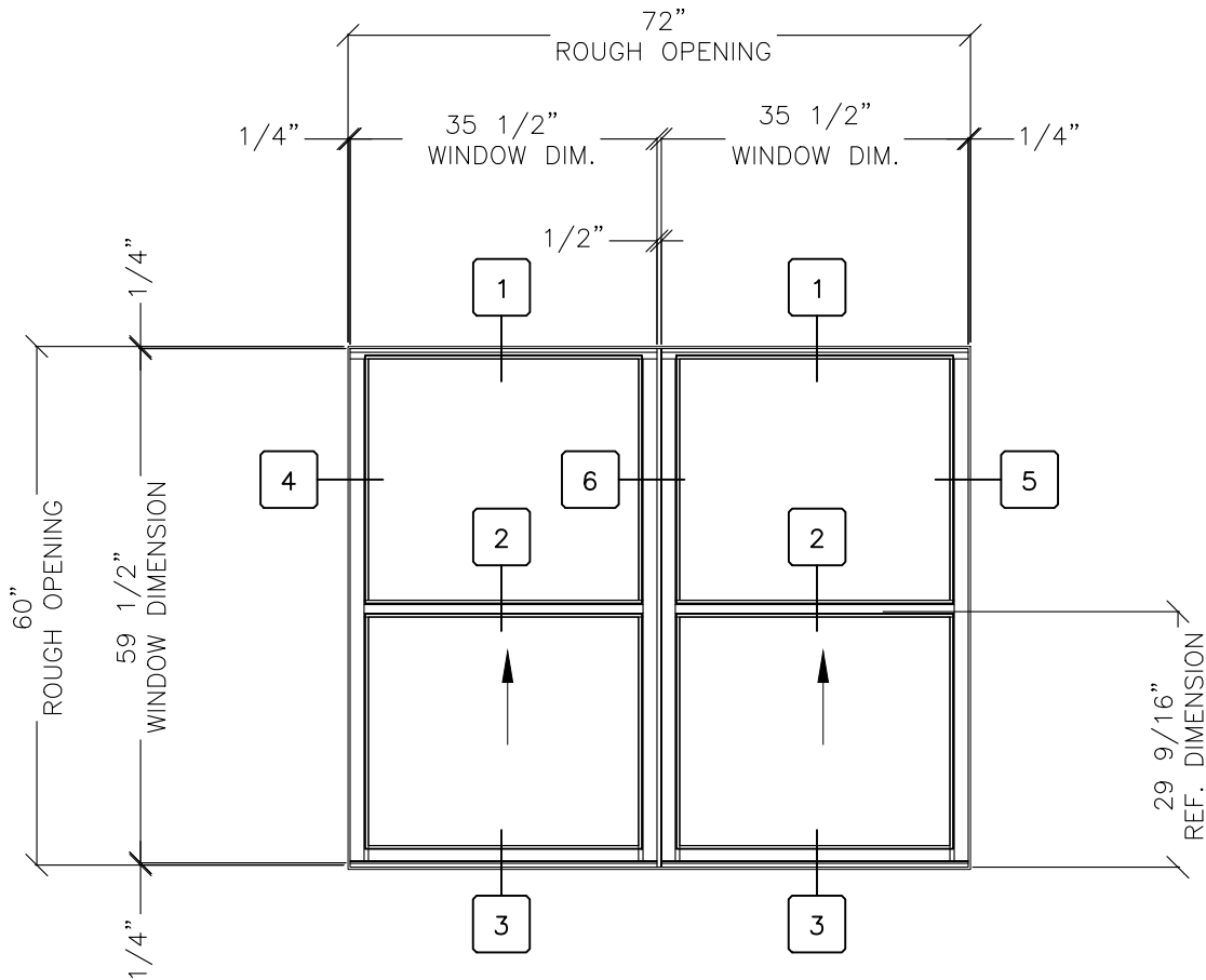
SINGLE HUNG / SINGLE HUNG
