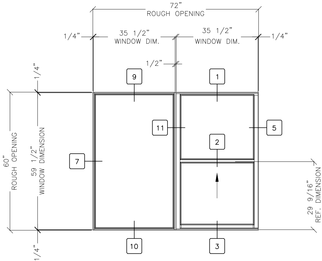
FIXED / SINGLE HUNG
